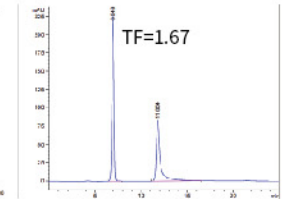
O-diphenol hydroxy naphthalene
