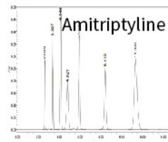
Peak tailing caused by acidic sites
